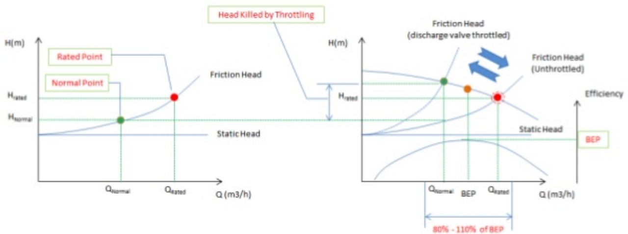
Fig-6: Pump Selection at Rated flow, BEP between Normal and Rated
