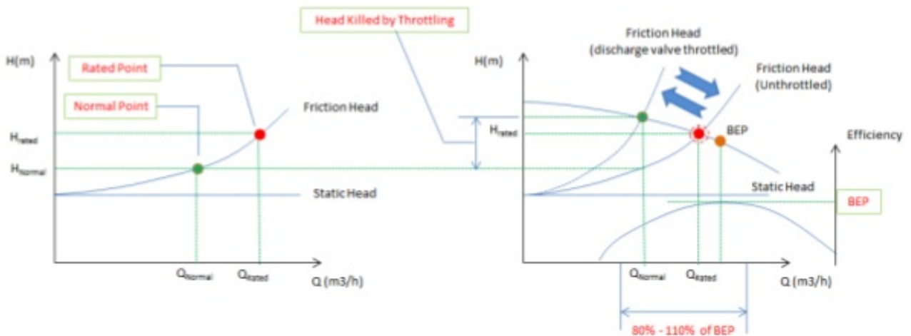
Fig-7: Pump Selection at Rated flow, BEP is NOT between Normal and Rated
